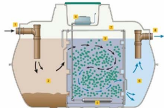
Sewage Treatment
